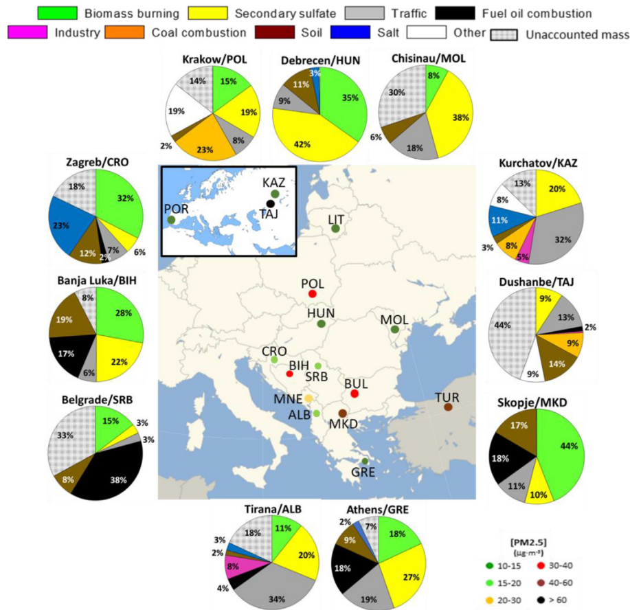
Fig. 2. Average contribution of PM 2.5 sources (values in %, 11 cities). Average measured PM 2.5 concentrations for the period of study (values in \mu\text{g}/\text{m}^3 , 16 cities).
